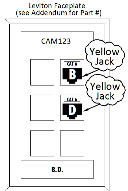
Camera Faceplate
