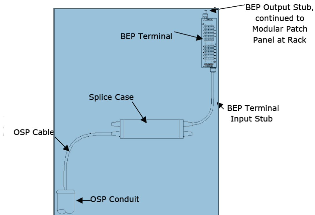
Backbone OSP Twisted Pair Cable Termination Example
